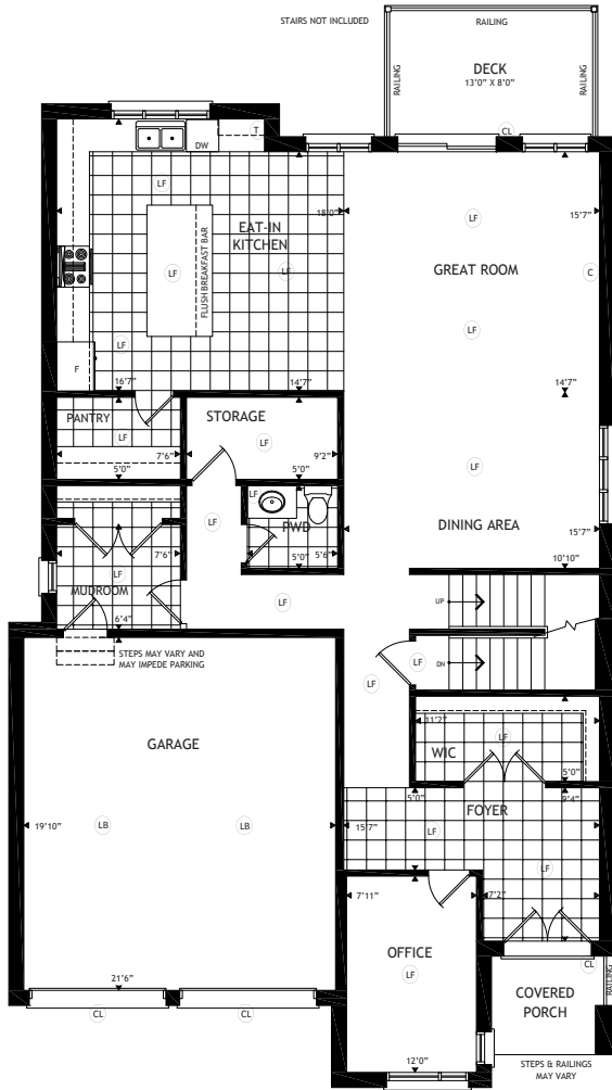
MAIN FLOOR
