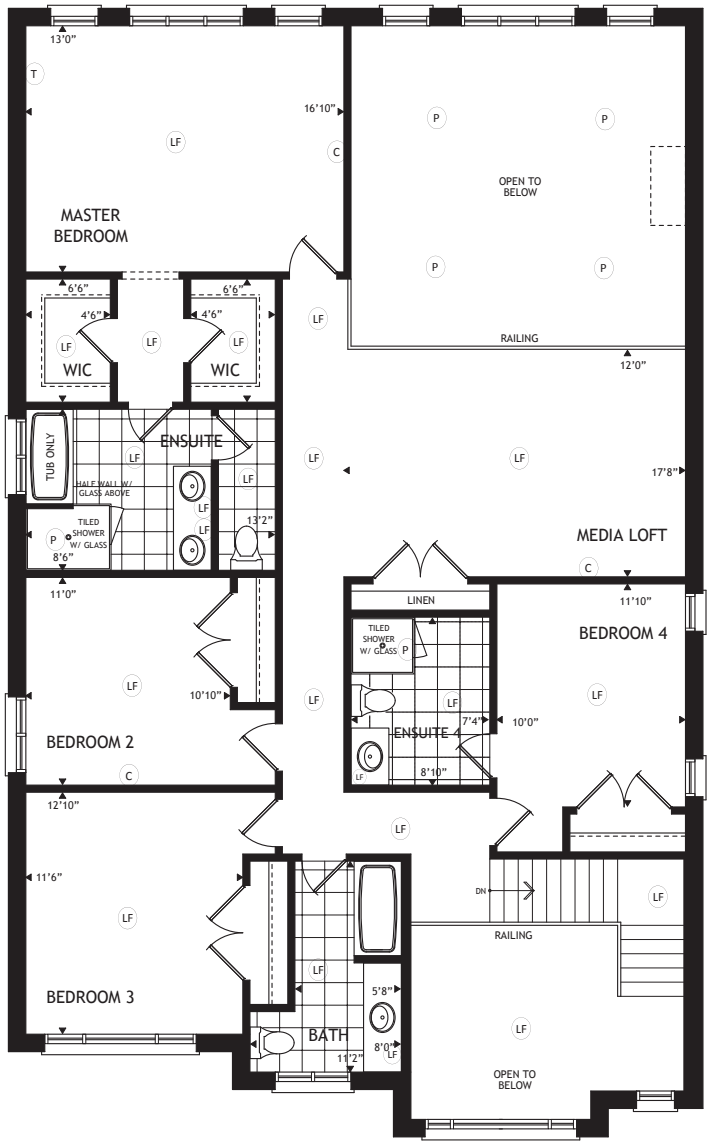
SECOND FLOOR
